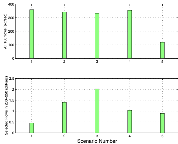
Fig. 6. Aggregate Throughput Performance of PCQoS
