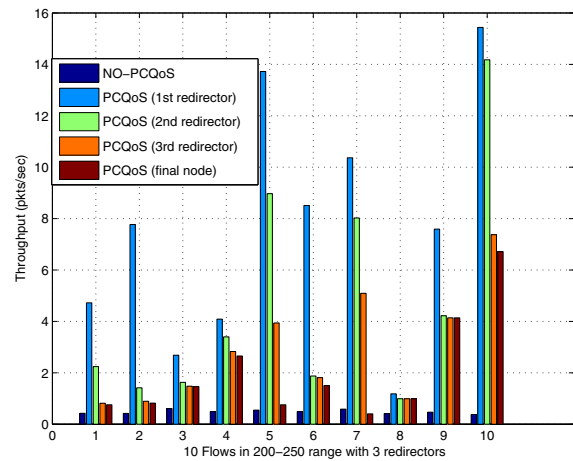
Fig. 5. Throughput Performance of 10 flows in the 200-250 meter range having 3 redirectors.
