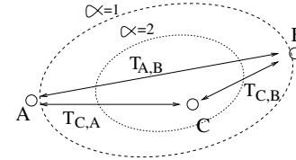
Fig. 3. Redirect Operation
