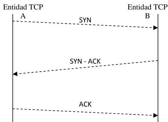
Figura 2.17 - 3-way handshake
